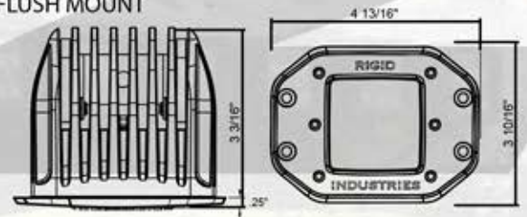
FLUSH MOUNT
